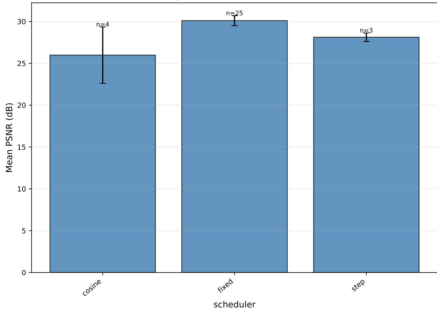
Mean PSNR per value of scheduler — SRFormer
